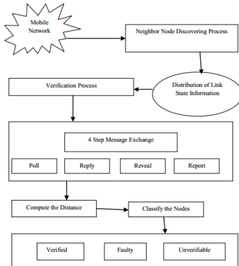
Figure 1. Architecture Diagram
