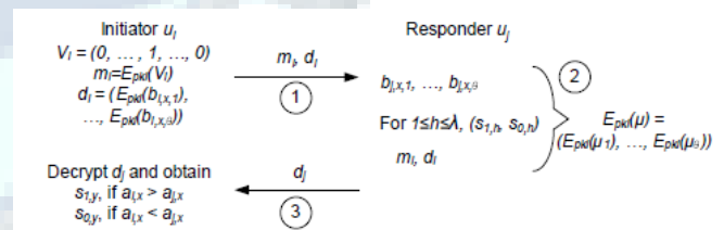
Fig 1. iCPM flow
