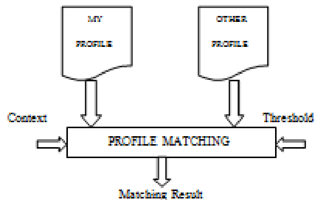
Fig. 3. Profile Matching
