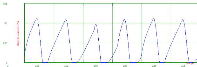
Fig. 20. Output current of IBFC with closed loop
