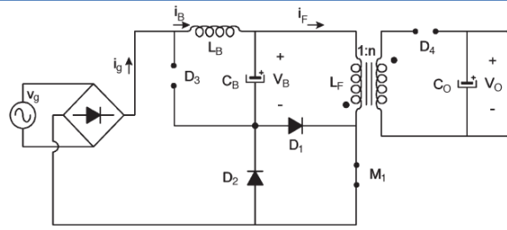
Fig. 7. Equivalent circuit of mode 2: v_g > V_B and M_1 is ON
