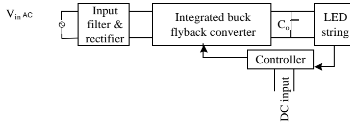
Fig. 4. Integrated single stage IBFC.
