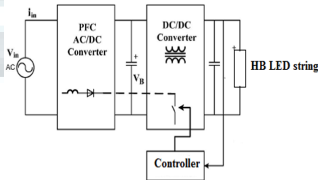
Fig. 3. Integrated single stage converter.
