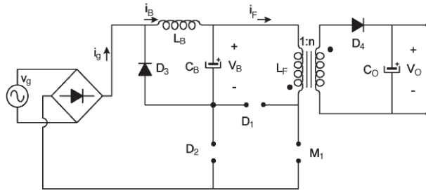
Fig. 8. Equivalent circuit during the conduction of M_1
