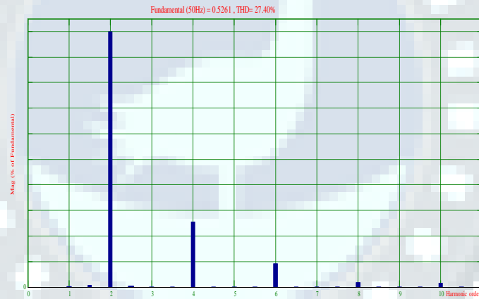
Fig. 17. THD spectrum of input current
