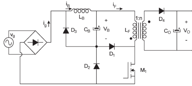
Fig. 5. Integrated buck flyback converter.
