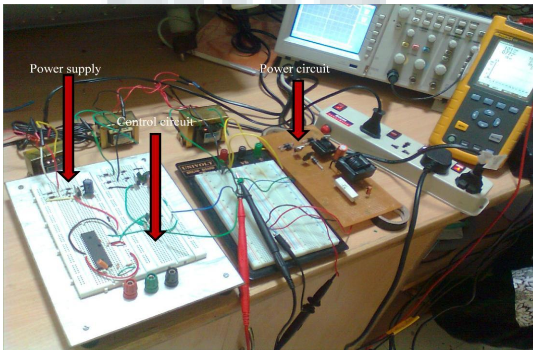
Fig. 21. Circuit setup of open loop IBFC
