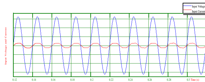
Fig. 19. Input voltage and current of IBFC with closed loop
