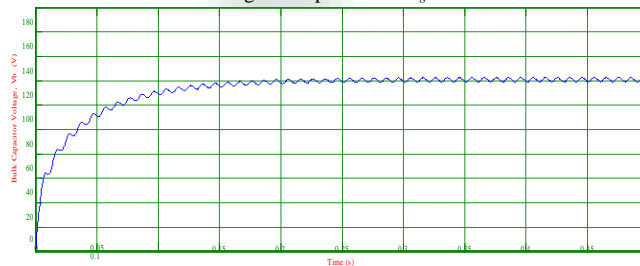
Fig. 14. Bulk capacitor voltage V_B
