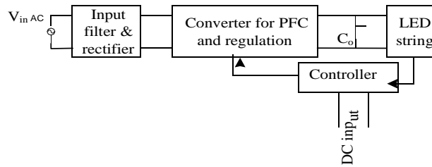
Fig. 1. Block diagram of single-stage power factor correction circuit
