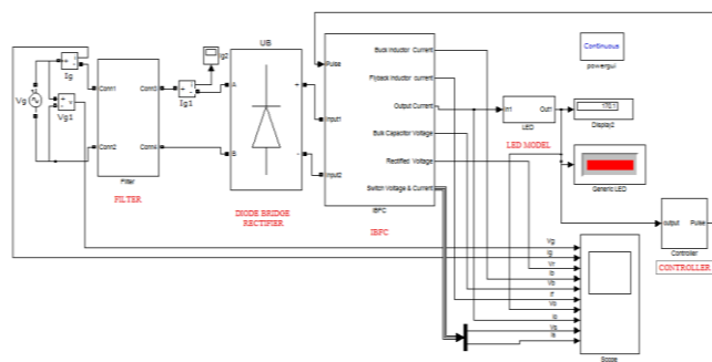
Fig. 18. Simulink model of closed loop IBFC used for streetlight application
