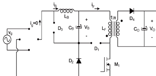
Fig. 6. Equivalent circuit of mode 1: v_g < V_B
