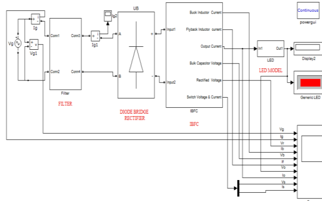
Fig. 11. Simulink model of open loop IBFC used for streetlight application
