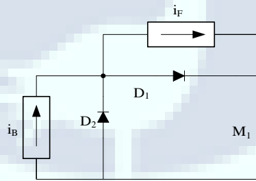
Fig. 8. Equivalent circuit during the conduction of M_1
