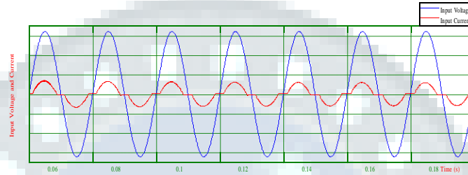
Fig. 16. Input voltage and current waveform
