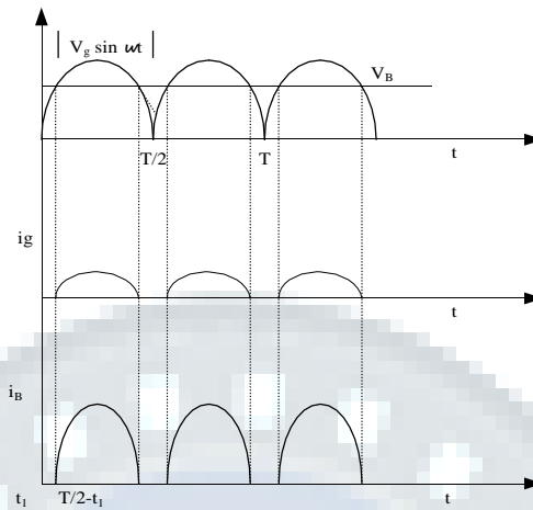
Fig. 10. Input voltage and current waveform of IBFC
