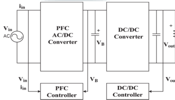
Fig. 2. Block diagram of two stage power factor correction circuit
