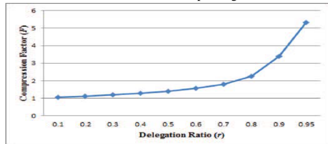
Fig 4. (A) Compression achieved by the tree-based approach for delegating different ratio of the classes
