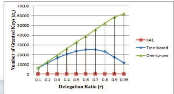
Fig 4. (B) Number of granted keys (na) required for different approaches in the case of 65536 classes of data.
