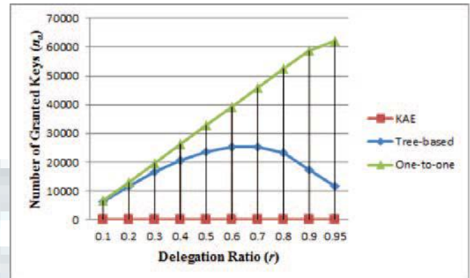
Fig 4. (B) Number of granted keys (na) required for different approaches in the case of 65536 classes of data.
