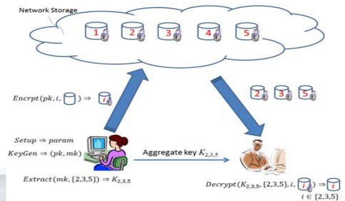
Fig2. Proposed KAC for data sharing in cloud storage system
